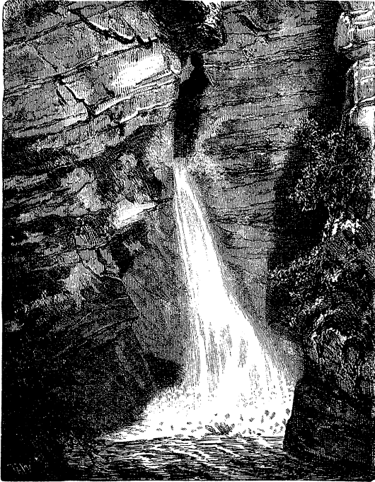
Fig. 3.—Structure of Sedimentary Rocks.
